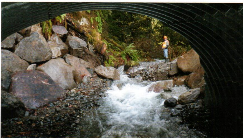
Large pipes with natural stream bottoms, called culverts, are used under roads in the watershed so that fish have access to their spawning streams.
